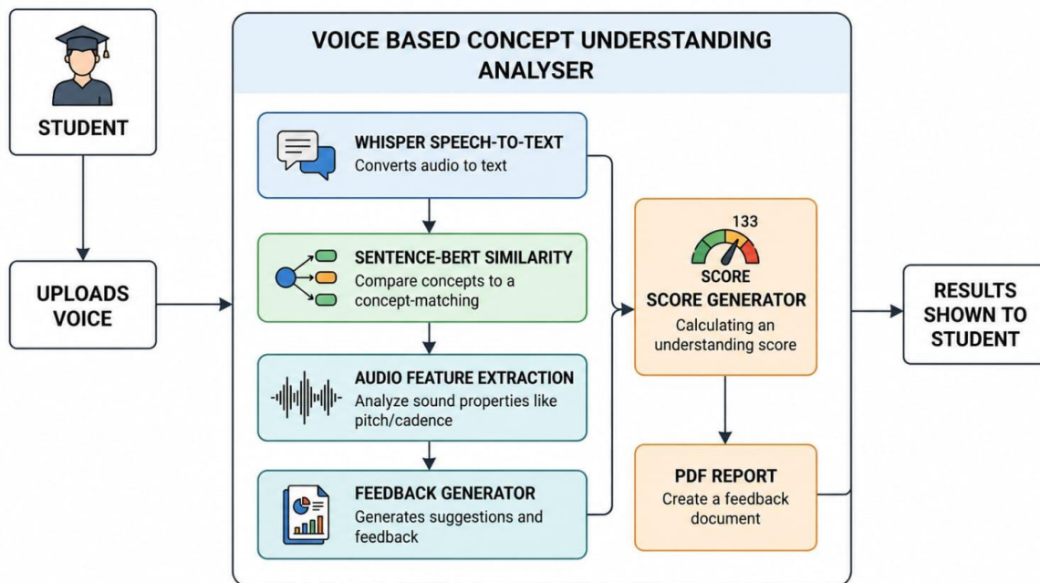
Figure 1: Data Flow Diagram of the Voice Based Concept Understanding Analyser
